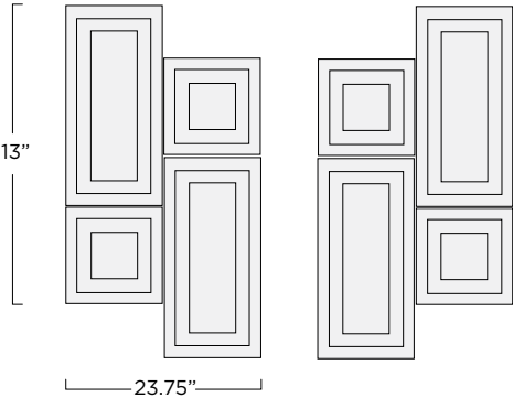
Tessellate 4 Sconce SC-352 (mirrored pair) SC-353 (single)
